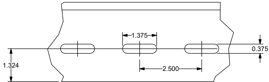
⑭ FENESTRATION DETAIL MAXIMUM OF 20 SLOTS PER SLAT MAXIMUM OF 2 SLATS SCALE: NTS
